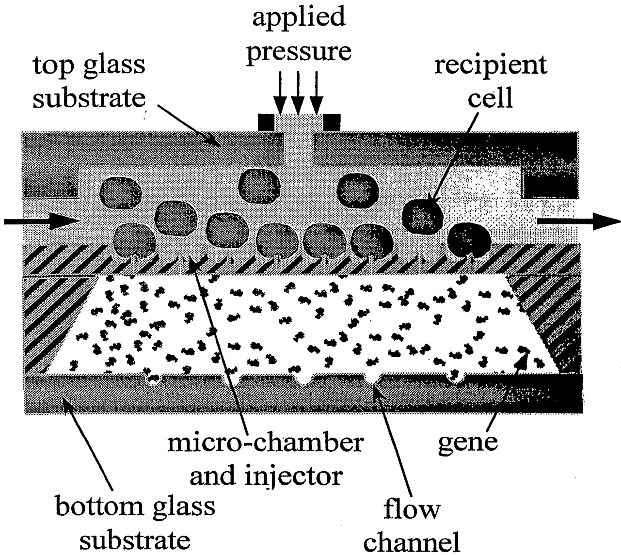
Fig. 1. Cell Transformation Microdevice
